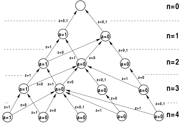
Figure G.1: Finite horizon policy graph structure.
