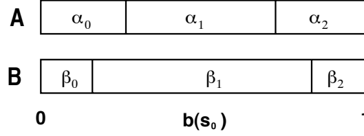
Figure 3.10: Partitions for PWLC sets A and B .
