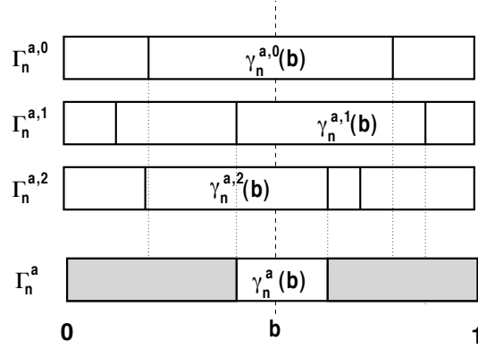
Figure 3.12: Defining the constraints on a region for Sondik's two-pass algorithm where \gamma_n^a(b) = \gamma_n^{a,0}(b) + \gamma_n^{a,1}(b) + \gamma_n^{a,2}(b) .
