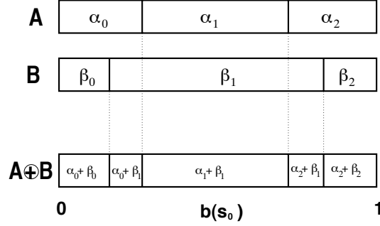
Figure 3.11: The final partition for A \oplus B and its relationship to the initial partitions of A and B .
