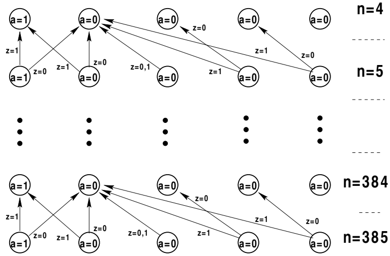
Figure G.3: Repeated policy graph structure.
